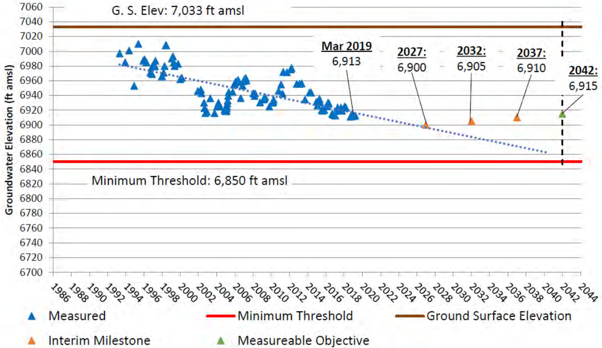
Figure 5-2. Groundwater Elevation Hydrograph, Sand Canyon Well #1
